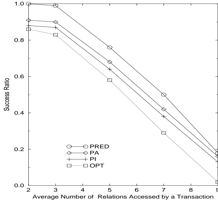
Fig. 5: Real-Time Performance Results under Varying Levels of Data Contention
