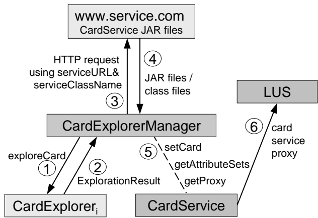
Figure 9. Download and instantiation of card services
